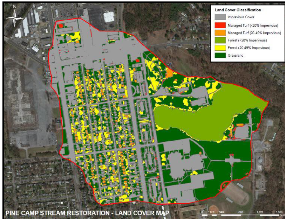
Figure 6-1. Drainage area and land coverage contributing to Pine Camp Creek stream.
