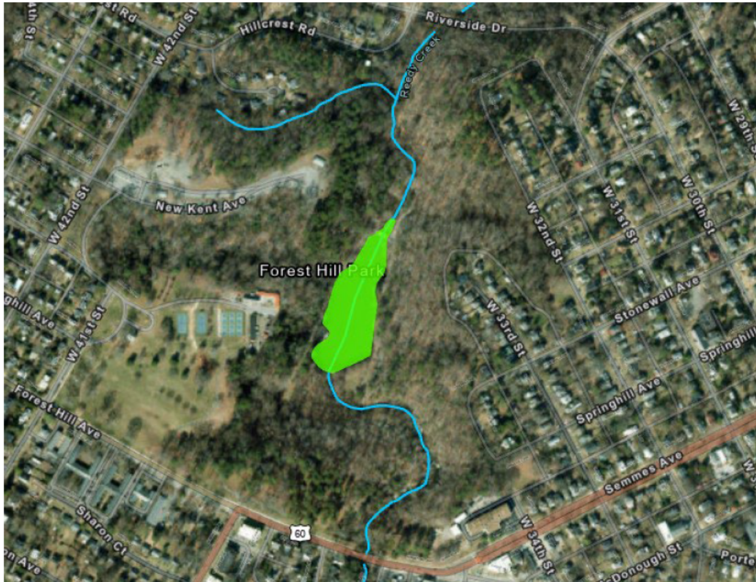
Figure 5-3. Forest Hill wet pond retrofit project location
