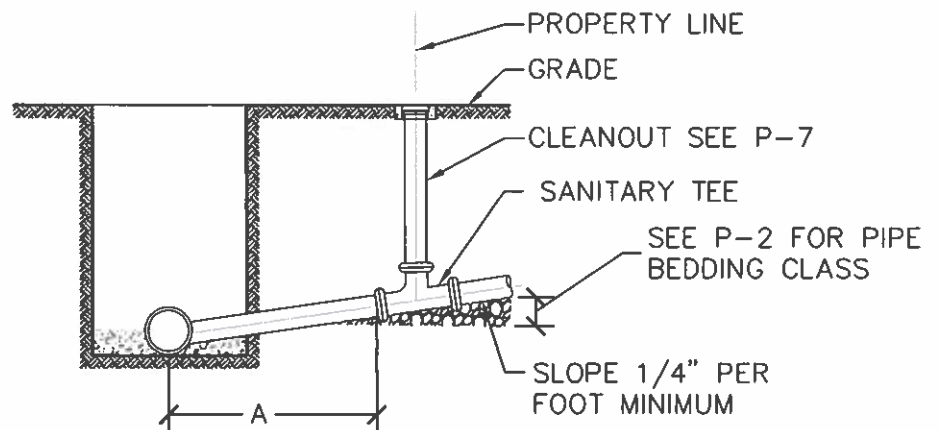
STANDARD LATERAL CONNECTION SECTION
