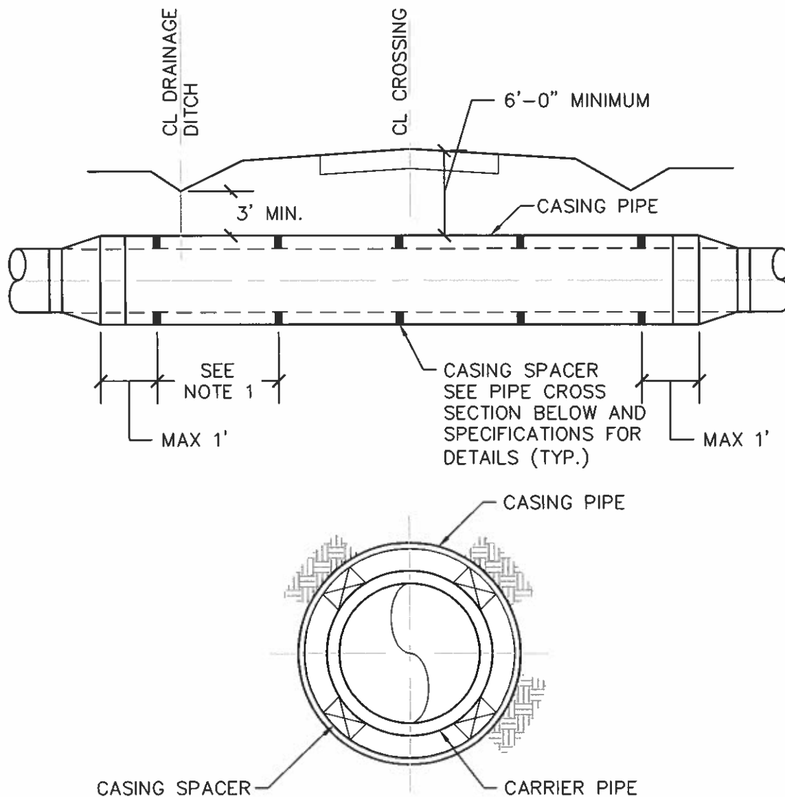
PIPE CROSS SECTION
