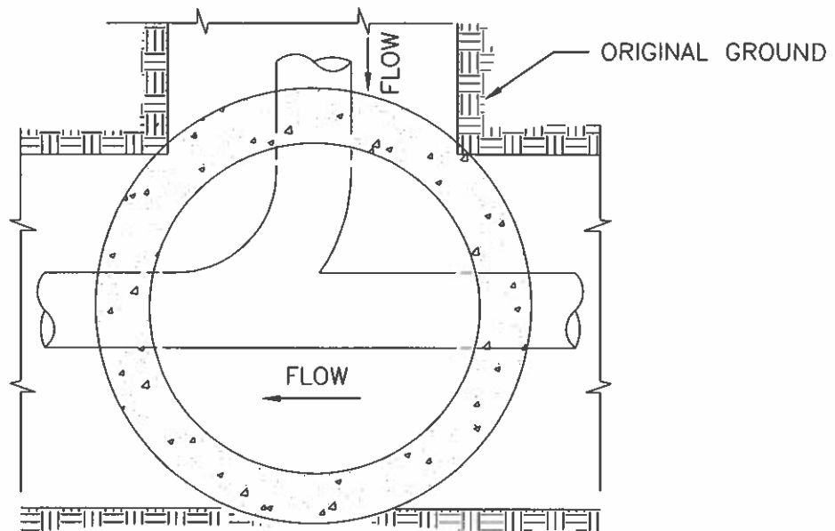
PLAN INVERT
