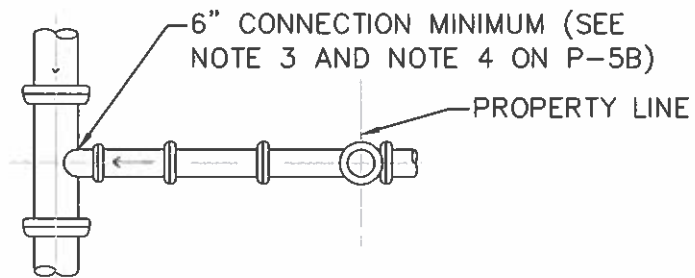
STANDARD LATERAL CONNECTION PLAN
