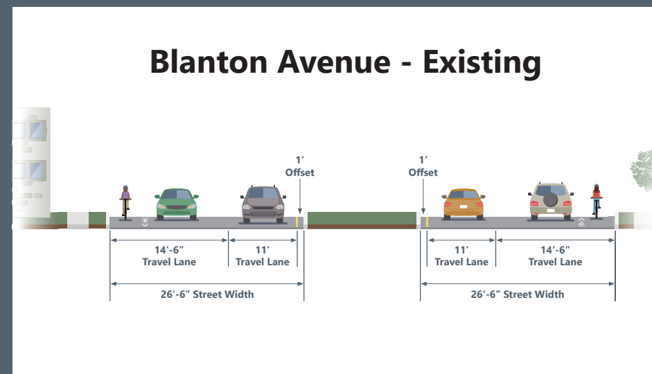
Blanton Avenue - Existing
