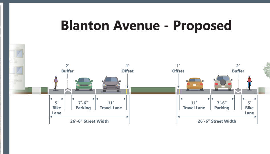
Blanton Avenue - Proposed
