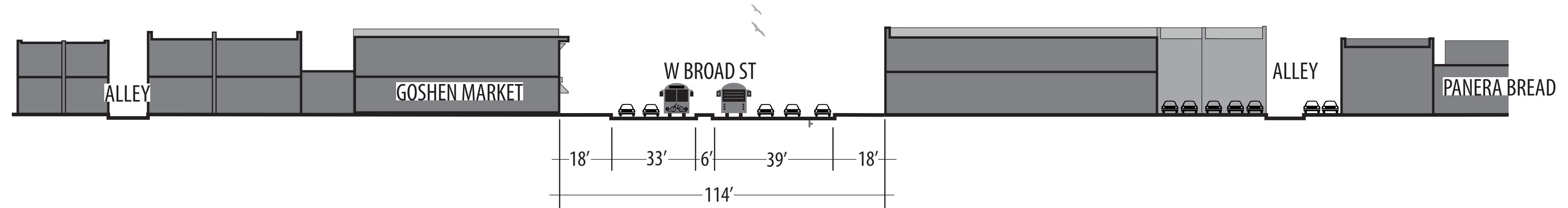
STREET SECTION - TODAY
